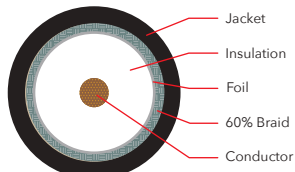
RG-6 60% DUAL SHIELD CMR/CMP
