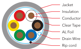
CONTROL 1806 SHIELDED
