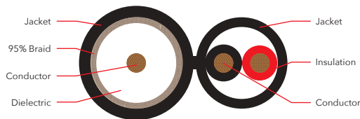
RG-59/BC + 18/2 BC
