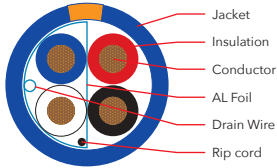
LUTRON-QS/M/500 & LUTRON-QS/M/1000
