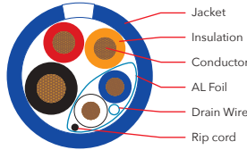
LUTRON-46/QSL/1000
