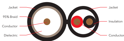
RG-59/CCS + 18/2 BC
