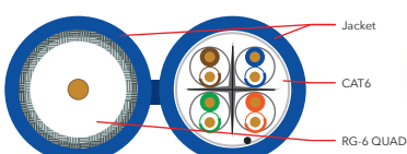
(1) CAT6 + (1) RG-6 QUAD
