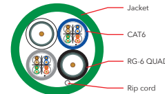
(2) CAT6 + (2) RG-6 QUAD
