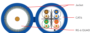
(1) CAT6 + (1) RG-6 QUAD
